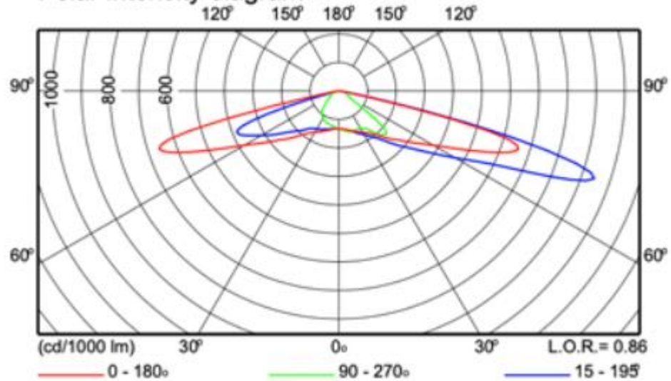
Polar intensity diagram
