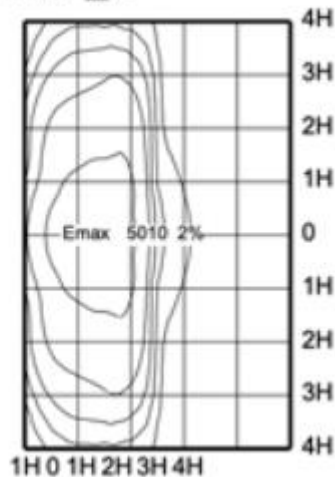
Horizontal Illuminance \triangle 0^\circ
