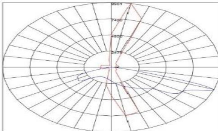
Maximum Candela = 9900.75 Located At Horizontal Angle = 80, Vertical Angle = 69.5 # 1 - Vertical Plane Through Horizontal Angles (80 - 260) (Through Max. Cd.) # 2 - Horizontal Cone Through Vertical Angle (69.5) (Through Max. Cd.)
