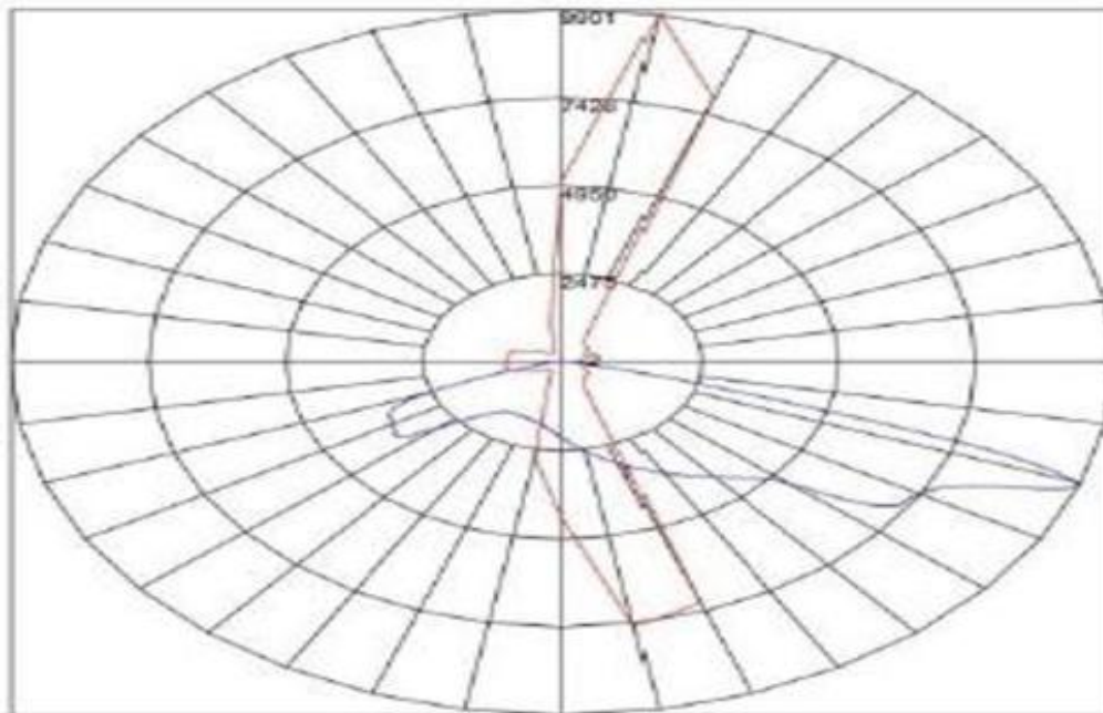
Maximum Candela = 9900.75 Located At Horizontal Angle = 80, Vertical Angle = 69.5 # 1 - Vertical Plane Through Horizontal Angles (80 - 280) (Through Max. Cd.) # 2 - Horizontal Cone Through Vertical Angle (69.5) (Through Max. Cd.)
